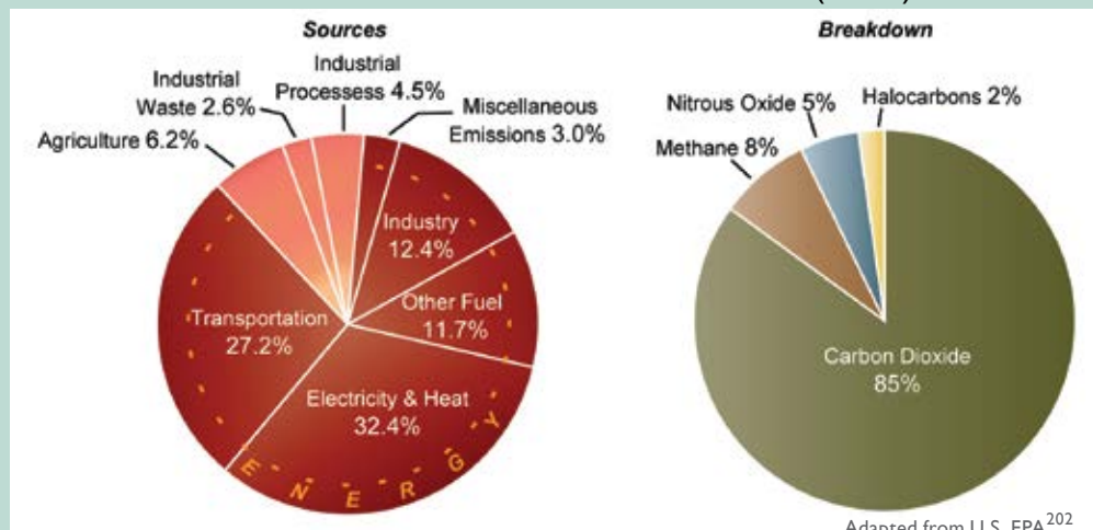
Sources of U.S. Greenhouse Emissions (2003)
